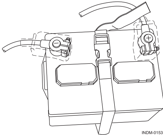
Figure 2.1 – Typical Marine Battery
