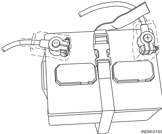
Figure 3.4 – Battery Connections
