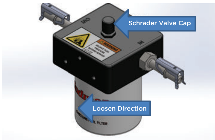
Figure 7.7 – Fuel Filter
