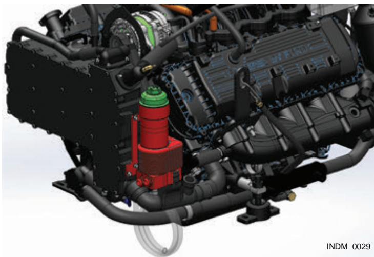
Figure 3.3 – Engine Oil Cartridge Filter
