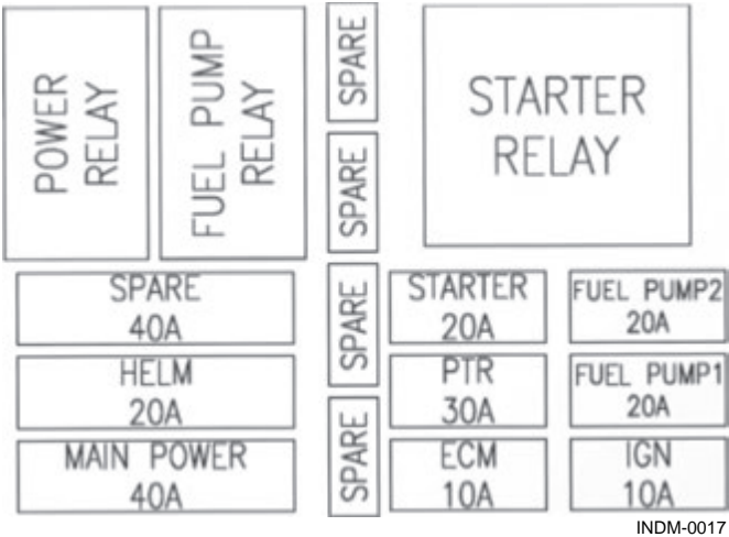
Figure 7.8 – Fuse Box Layout
