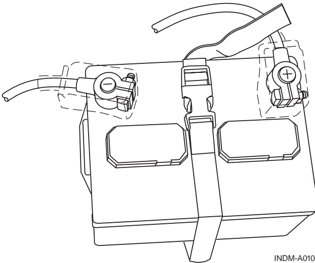
Figure 3.4 – Battery Connections
