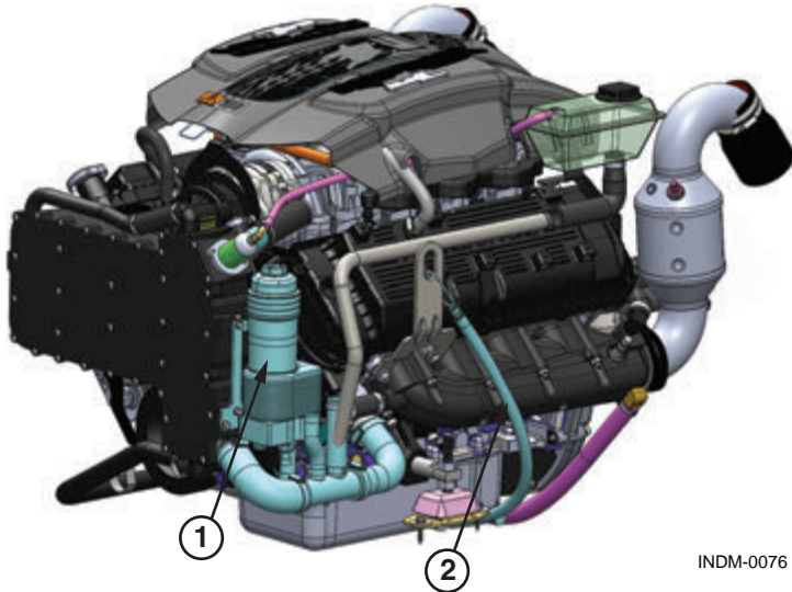
Figure 7.4 – Oil Filter and Drain
