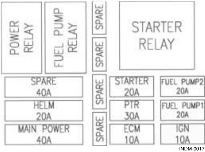
Figure 7.8 – Fuse Box Layout
