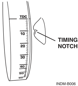
Figure 6.10 – Timing Notch
